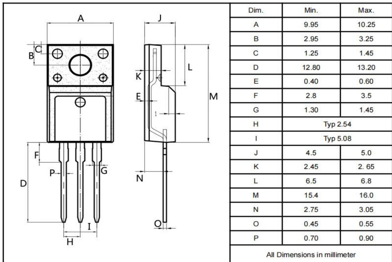
TO-220F
