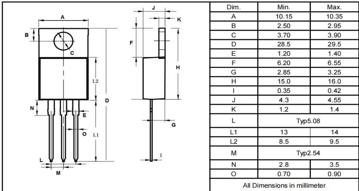
TO-220AB
