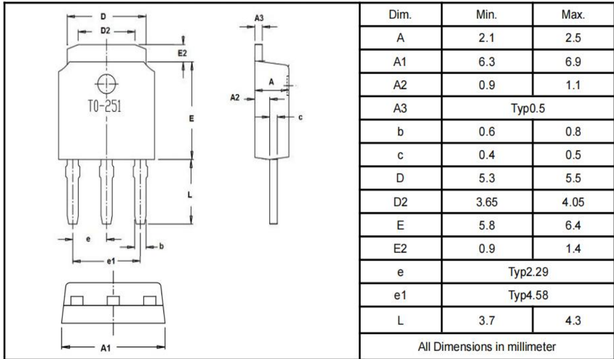
TO-251
