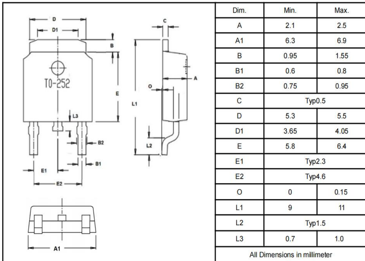
TO-252
